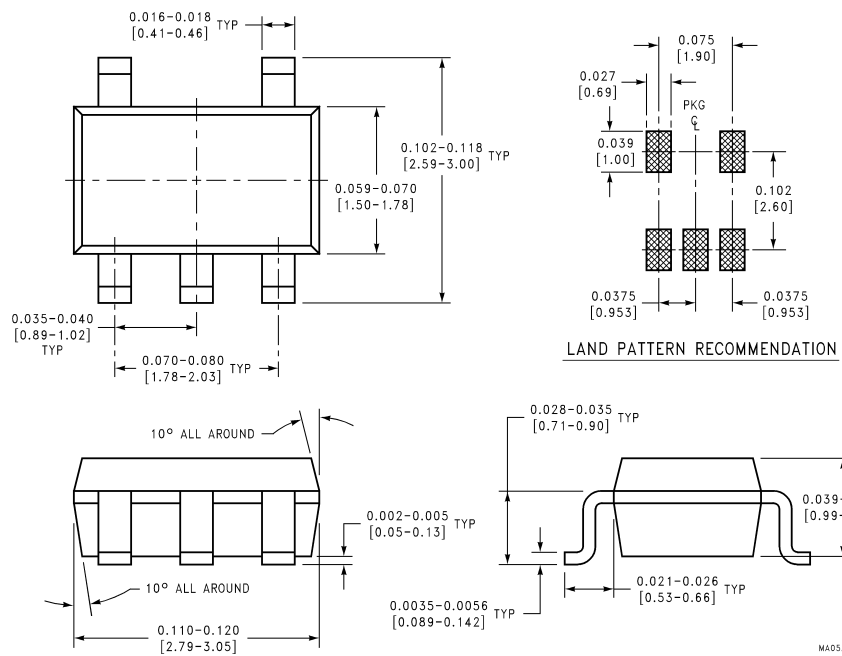
5-Lead Molded SOT23-5 Order Number LM7121IM5 or LM7121IM5X NS Package Number MA05A
